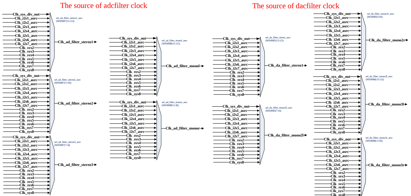
Figure 11. Digital ADC/DAC Filter Clock Tree
