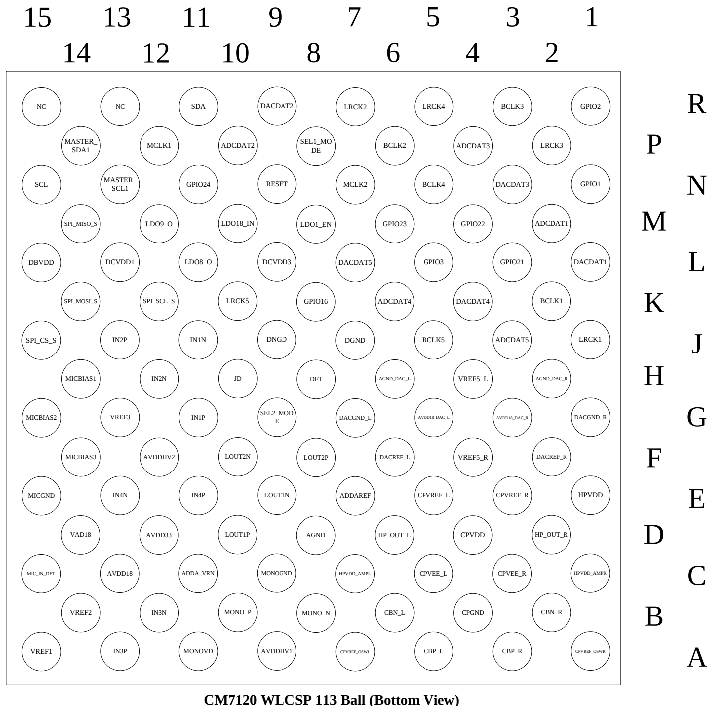
Figure 4. Pin Assignments
