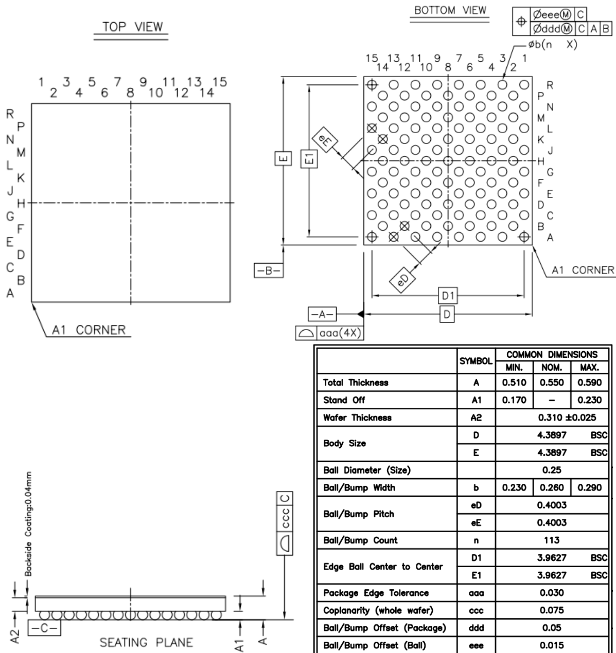
Figure 59. Package Dimension
