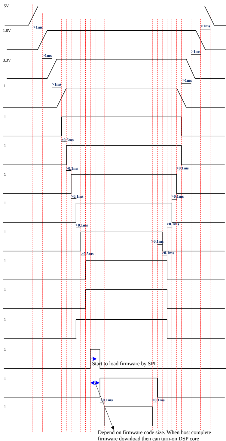
Figure 5. Power On/Off Timing when Normal Load Code by SPI Interface
