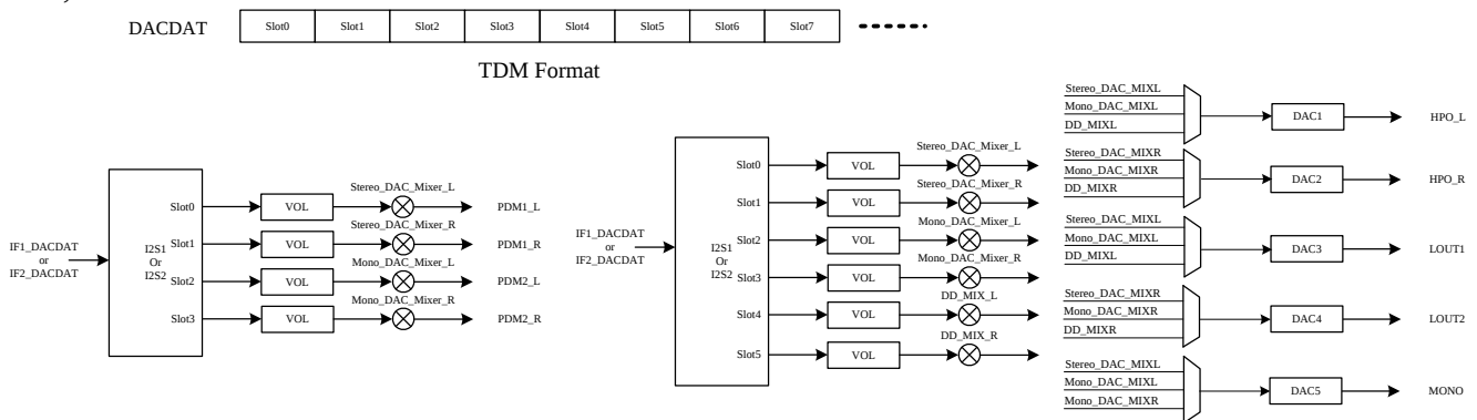
Figure 35. Multi-Channel Playback Path
