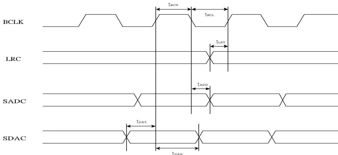
Figure 55. Timing of I2S/PCM Slave Mode
