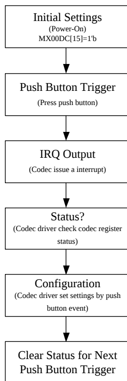
Figure 49. 3 Push Button Detection Flow
