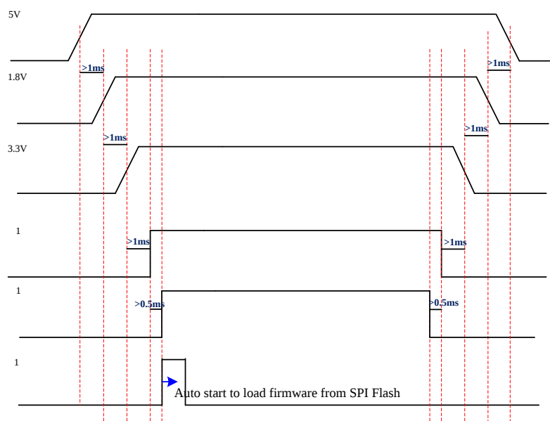
Figure 6. Power On/Off Timing when Normal Load Code by SPI Flash
