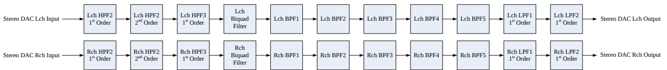
Figure 40. EQ Structure on the Playback Path
