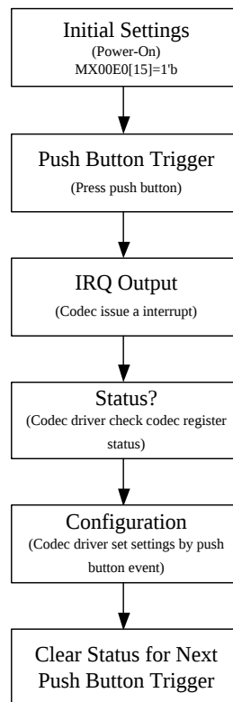
Figure 50. 4 Push Button Detection Flow
